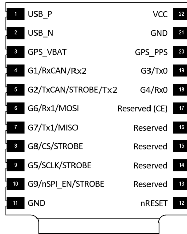
μIMU, μAHRS, μINS Module - Top View
