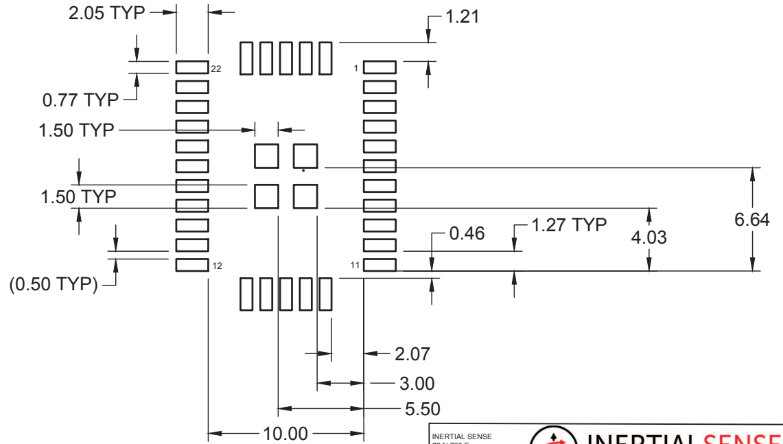
RECOMMENDED FOOTPRINT
