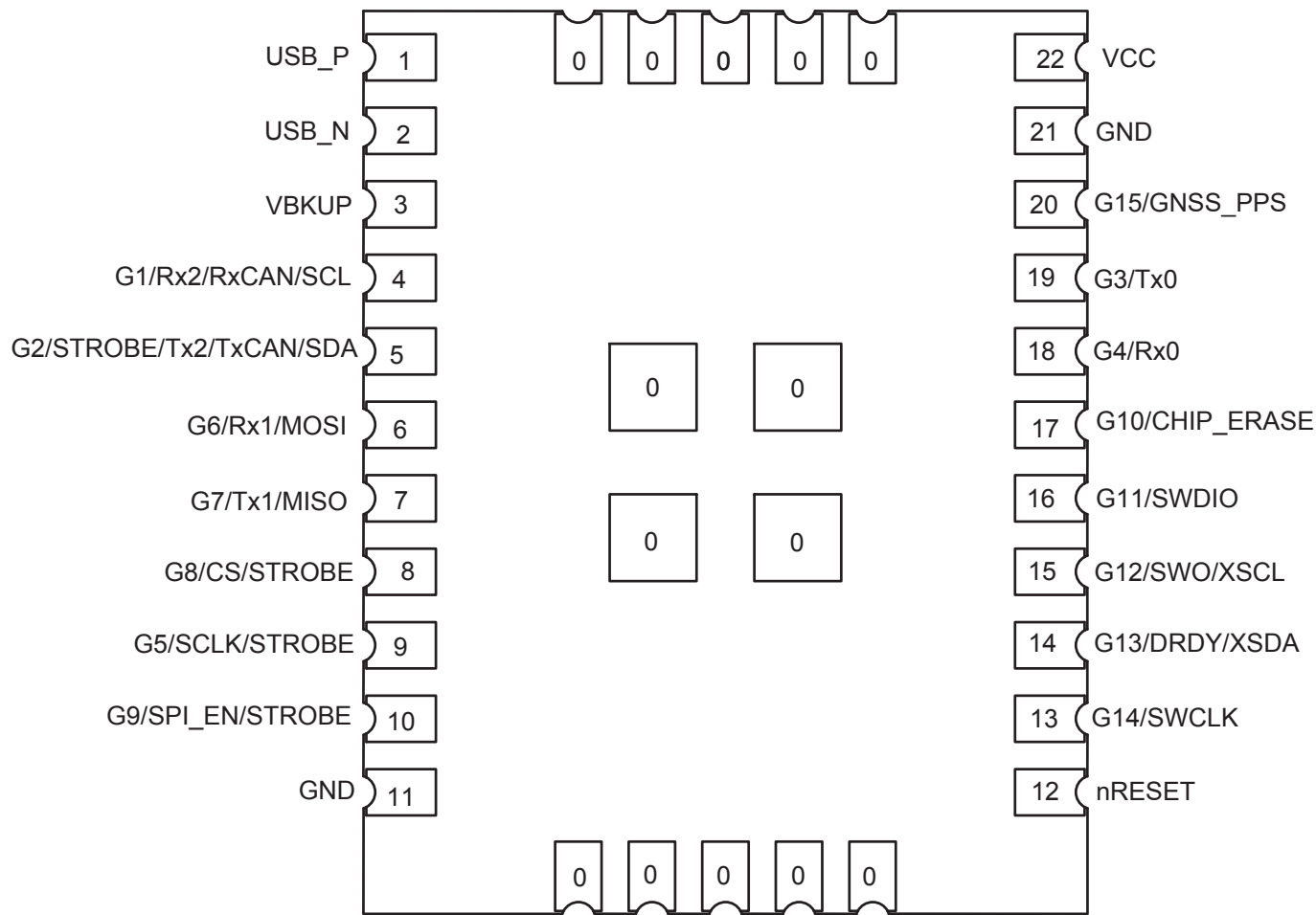
TOP VIEW
