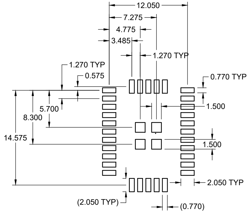
RECOMMENDED FOOTPRINT
