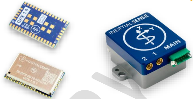
GPX-1 Size: 20.7 x 12.5 x 2.9 mm Weight: 1.7 g GNSS: Multi-Band L1/L5
